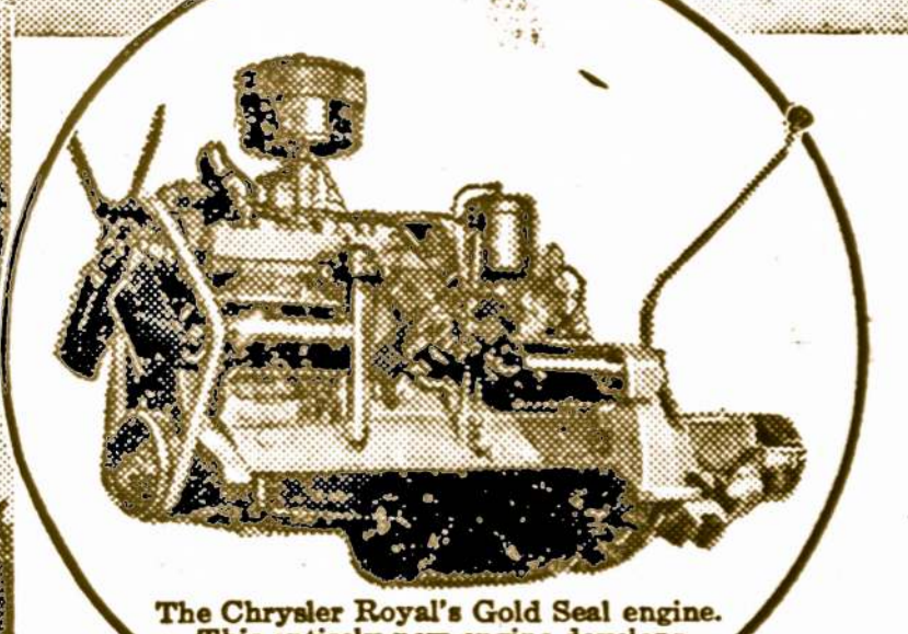
The Chrysler Royal's Gold Seal engine. This entirely new engine develops 93 h.p. with a piston displacement of but 228.1 cu. in.
